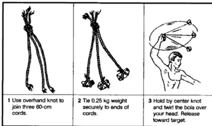
Figure 12-7. Bola.
