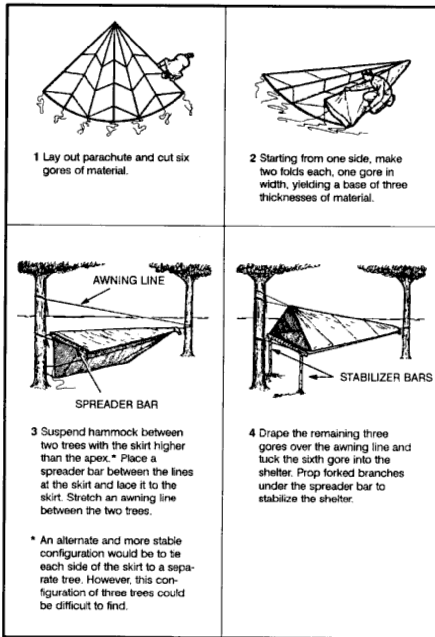
Figure 5-8. Parachute hammock.
